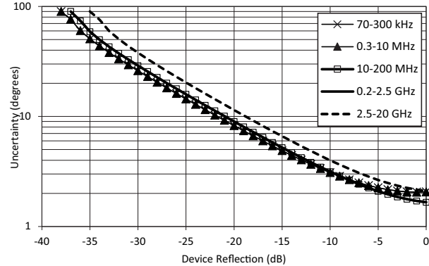
Reflection Phase Uncertainty; MS4642B (Opt. 8/9); SOLT Calibration using 3652A K Cal Kit
