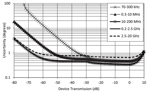
Transmission Phase Uncertainty; MS4642B (Opt. 8/9); SOLT- SL Calibration using 3652A -1 K kit
