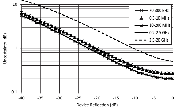
Reflection Magnitude Uncertainty; MS4642B (Opt. 8/9); SOLT Calibration using 3650A 3.5mm Cal Kit
